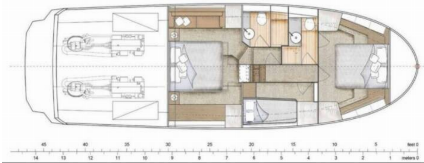
GREENLINE 45 FLY - LOWER DECK WITH THIRD CABIN
