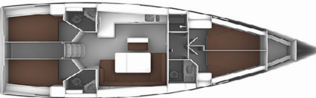
Bavaria Cruiser 46 - 4 cabin layout
