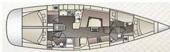
Deck plan diagram of the Elan 444 Impression sailboat.
