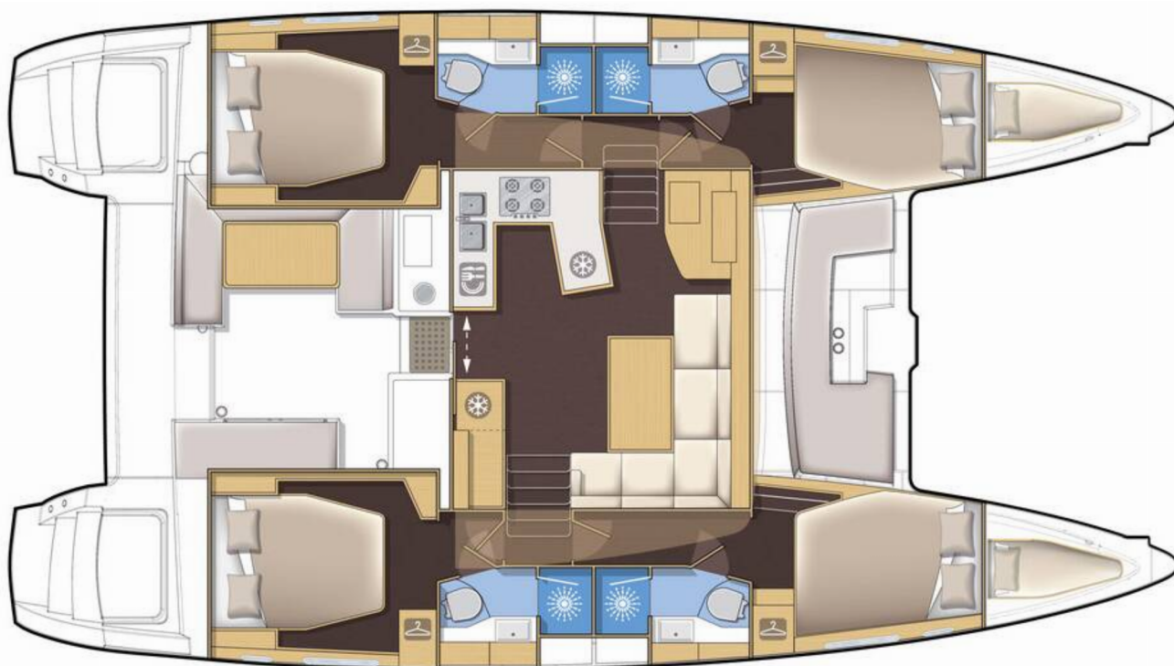
Version 4 cabins / 4 cabin version
