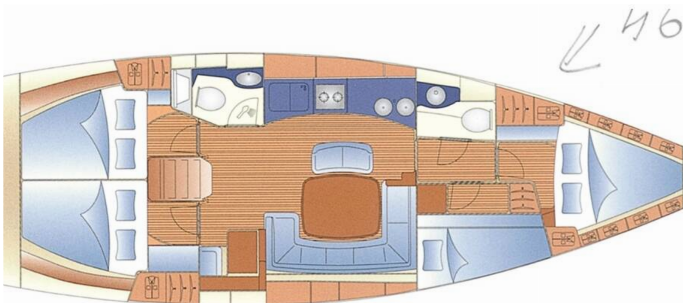
Kabinen Version / 4-Cabin version
